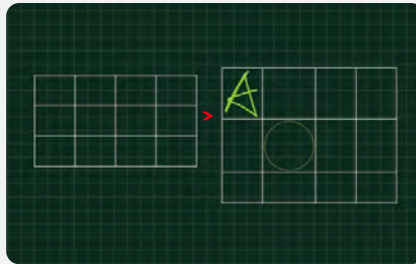
Dynamic table
