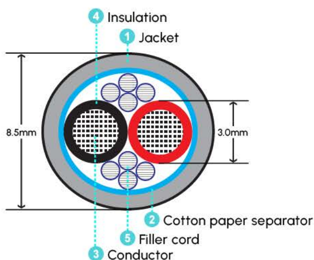
Maier speaker cable speakon MSC Series range of loudspeaker connectors.
